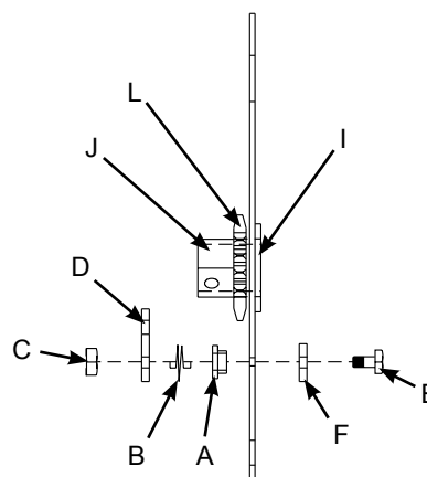
Side View of Tarp Housing
